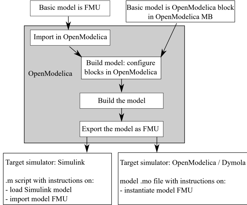
Figure 4.8: Basic steps for generating a model FMU and its preparation for a target simulator.
