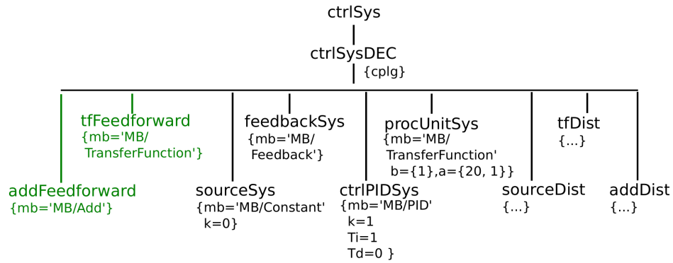
Figure 3.5: FPES for PES number 2 in Figure 3.4.
