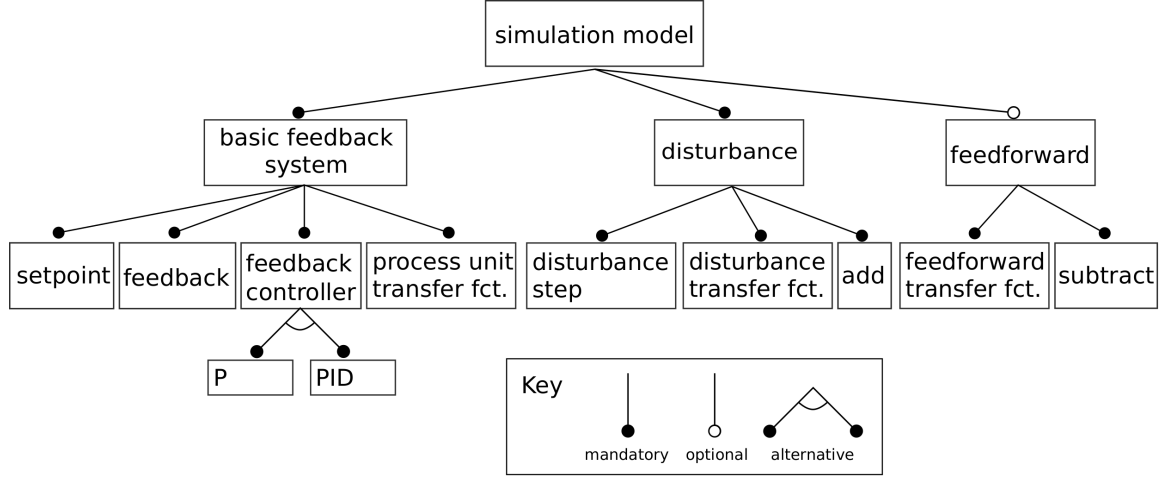
Figure 2.12: FM for specification of variants of a simple control system.
