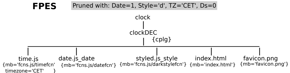
Figure I.3: A possible FPES of a HTML / JavaScript clock.
