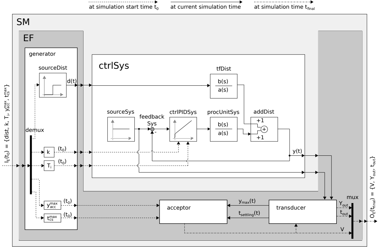
Figure 3.13: Structure of an SM consisting of an EF and the model structure of the feedback control system without feedforward control as MUS.
