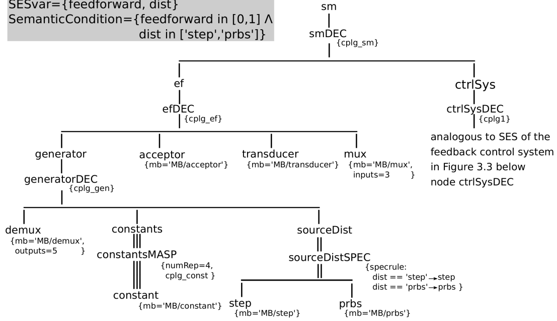
Figure 3.14: SES of the feedback control system as MUS and appropriate EF.
