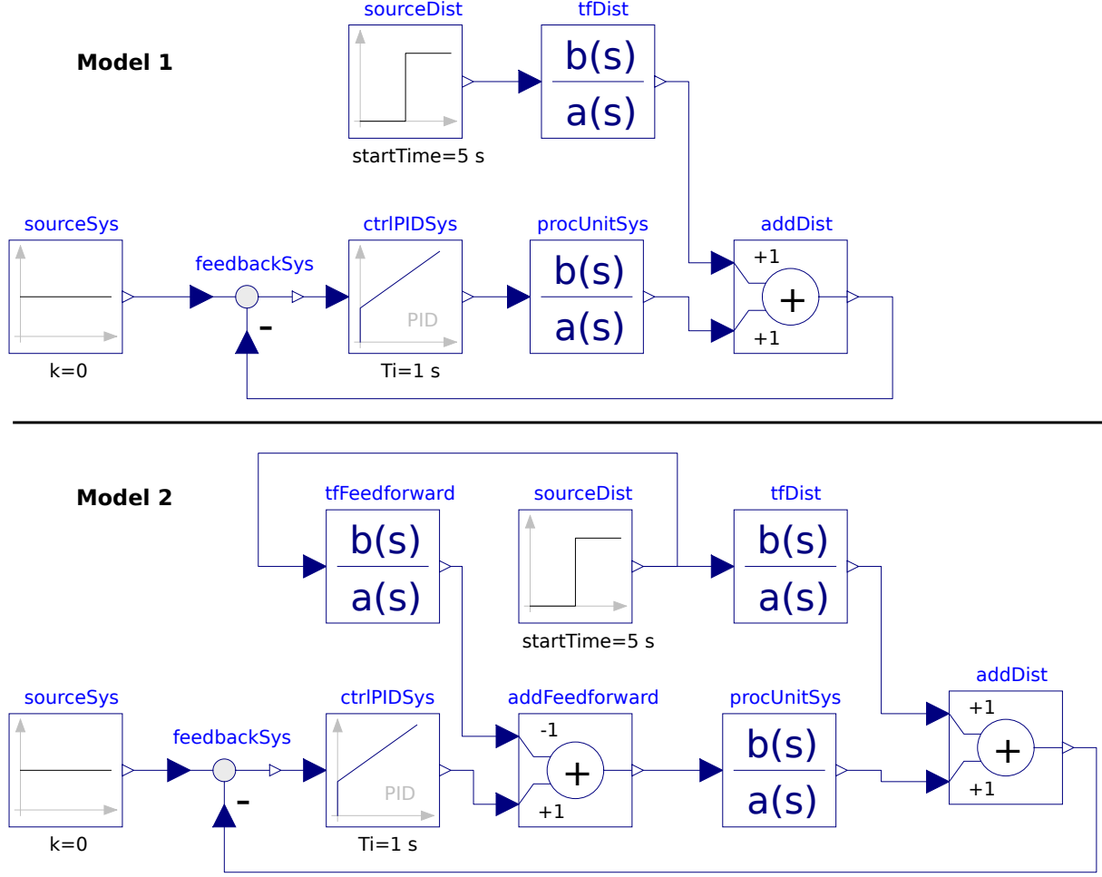
Figure 3.7: Modelica-based model structures generated with the build operation and using an FPES: (i) case \text{feedforward} = 0 \rightarrow without feedforward control and (ii) case \text{feedforward} = 1 \rightarrow with feedforward control.
