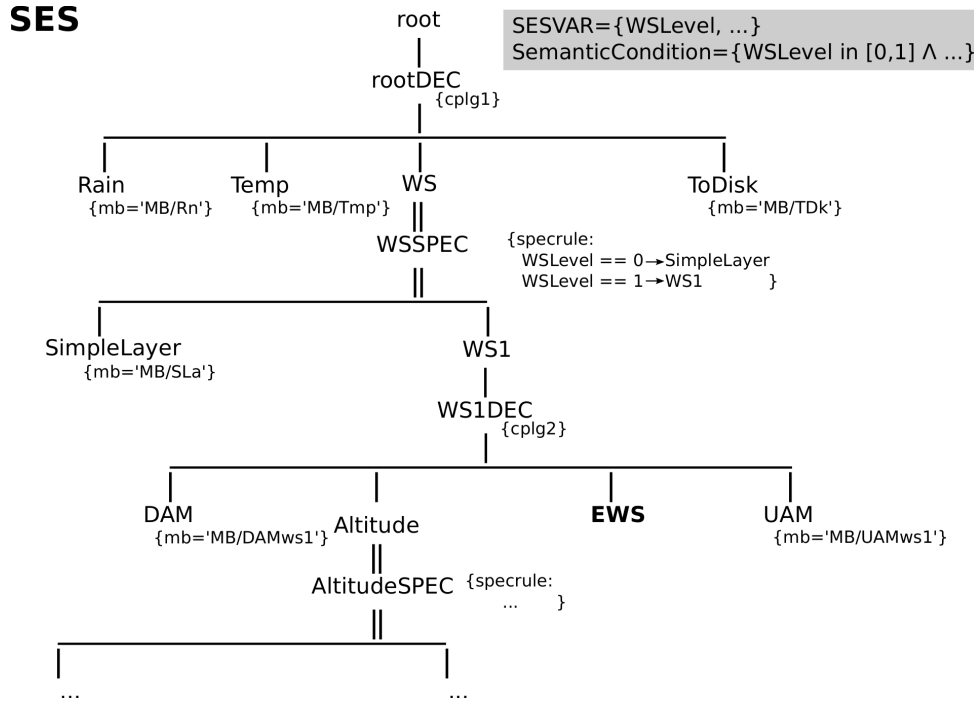
Figure 5.1: An excerpt of the SES for specifying model variants of the watershed with model components of different levels of detail.
