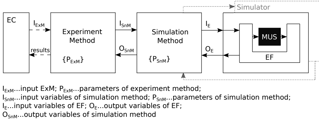
Figure 3.15: Block diagram for structuring complex simulation-based experiments according to Schmidt [135] with supplemented interface to an EC.
