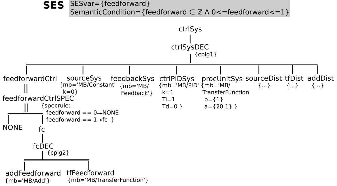
Figure 3.3: SES of the feedback control system.
